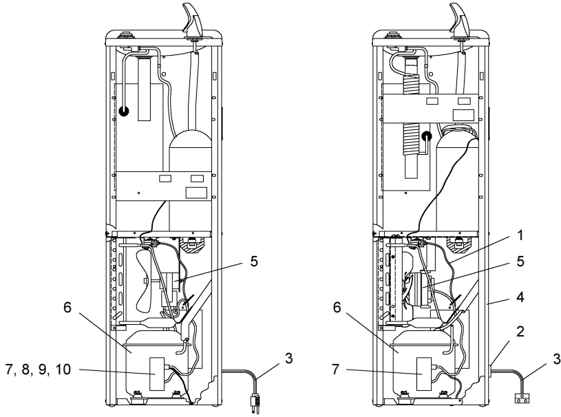
FD7003, 5, 8, & 10 LFDE8
