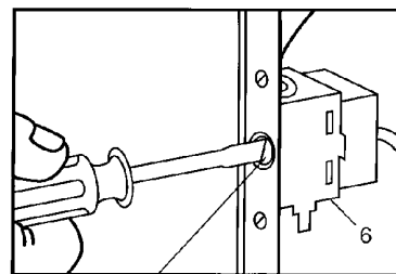
Cold Thermostat Adjustment Clockwise - For Colder Water
