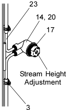
Stream Height Adjustment Detail
